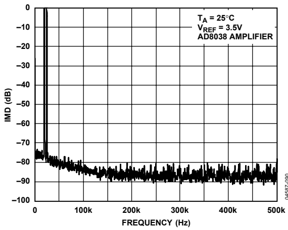
Figure 40. Wideband IMD, f_{OUT} = 20\text{ kHz}, 25\text{ kHz}, \text{Clock} = 1\text{ MHz}
