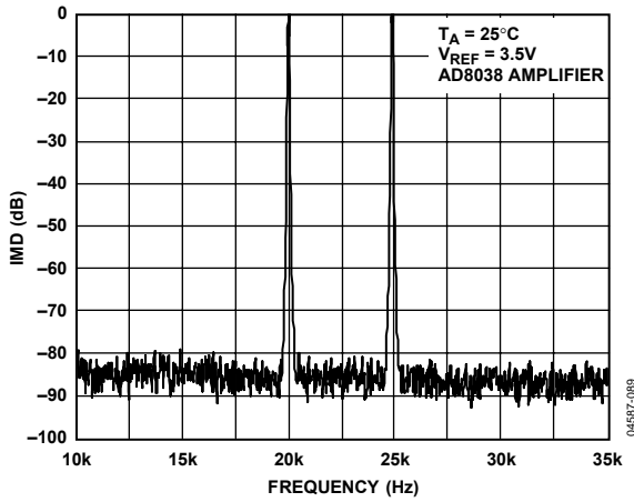
Figure 39. Narrow-Band IMD, f_{OUT} = 20\text{ kHz}, 25\text{ kHz}, \text{Clock} = 1\text{ MHz}
