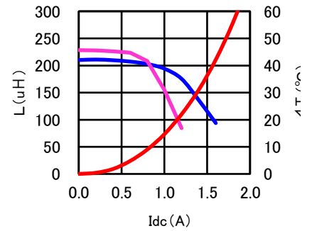
CDRH10D60BT150NP-221MC
