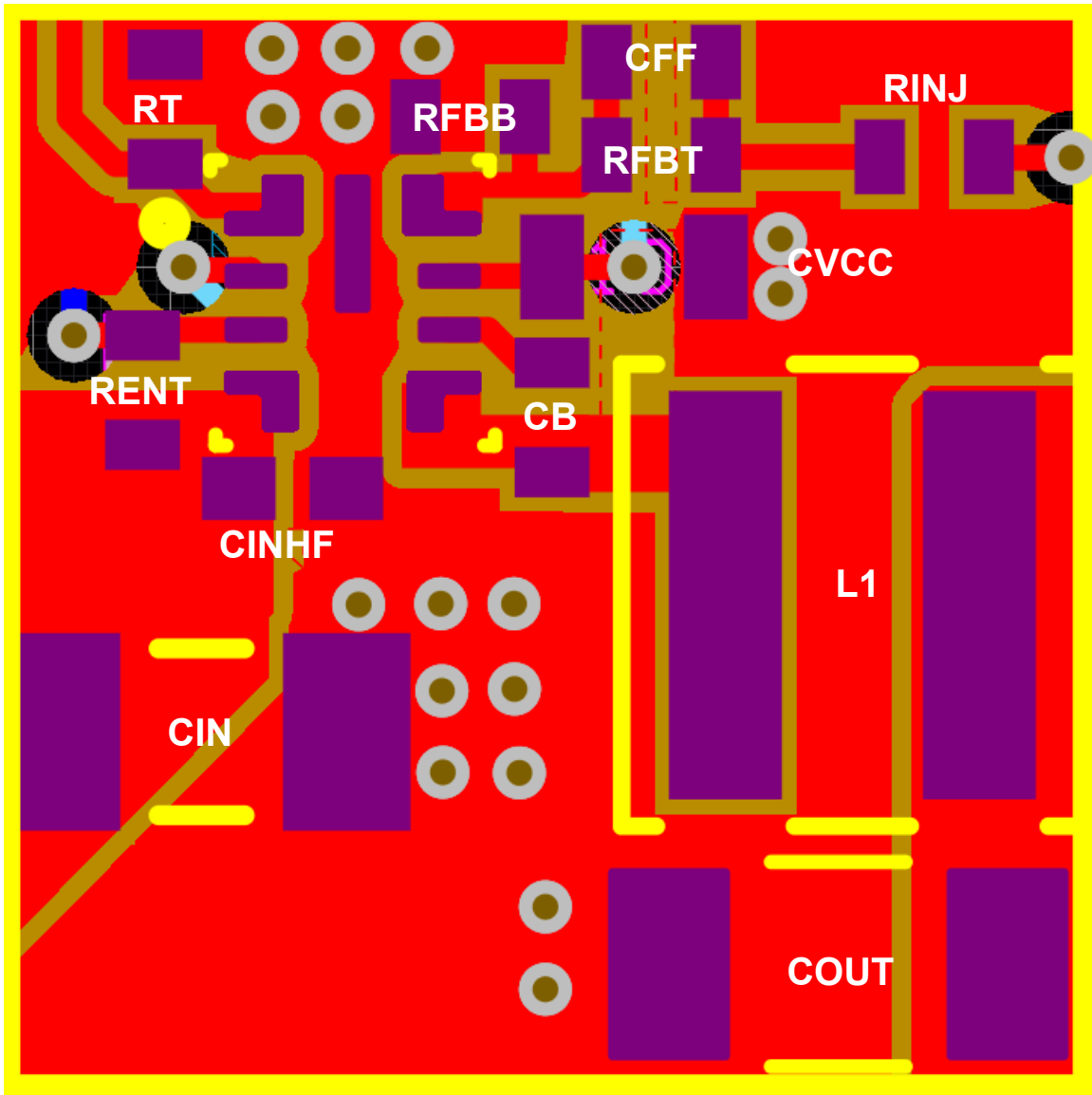
Figure 8-32. Example Layout
