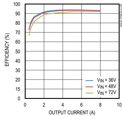
EFFICIENCY CURVES
