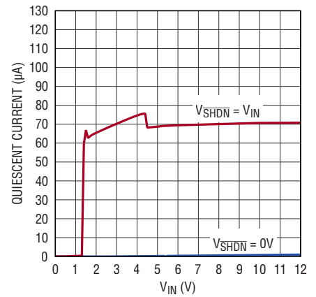
LT3066-5 Quiescent Current
