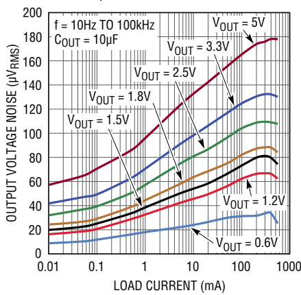
RMS Output Noise vs Load Current vs C_{\text{REF/BYP}} = 10\text{nF} , C_{\text{FF}} = 0
