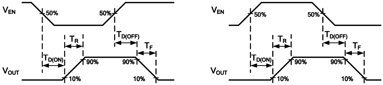
Figure 1 Voltage Waveforms: AP2401A (left), AP2411A (right)
