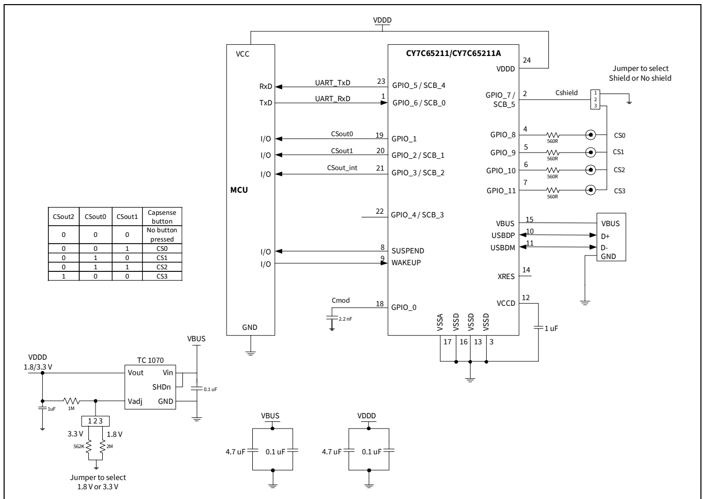
Figure 13 CAPSENSE™ schematic
