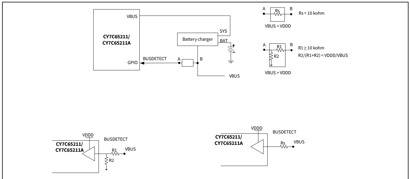
Figure 10 9 V tolerant
