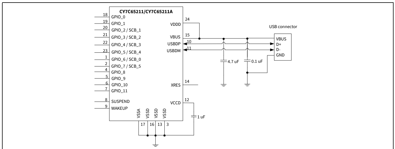
Figure 3 Bus-powered configuration
