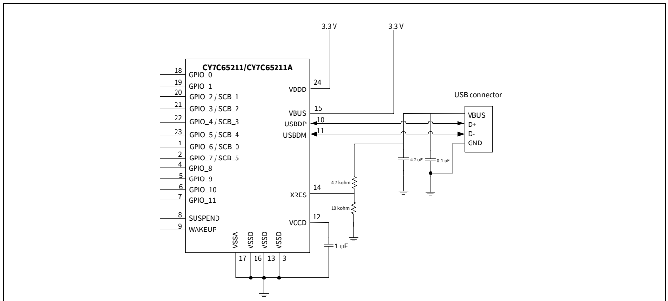
Figure 4 Self-powered configuration
