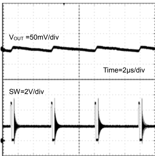
Figure 29. SW Waveform (SLLM™ Control) ( V_{IN} = 5.0\text{V} , V_{OUT} = 1.8\text{V} , I_{OUT} = 50\text{mA} )
