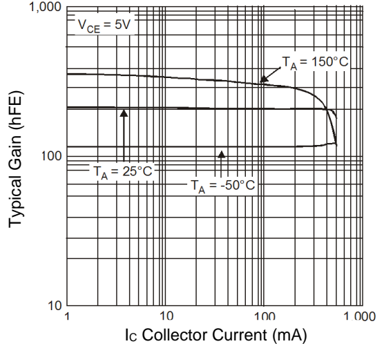
Figure 5. h_{FE} \text{ v } I_C
