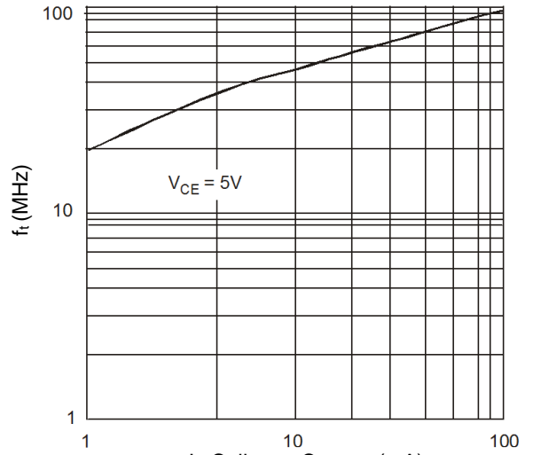
Figure 7. f_t \text{ v } I_C
