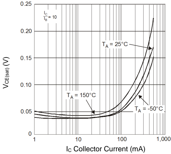
Figure 4. V_{CE} \text{ v } I_C
