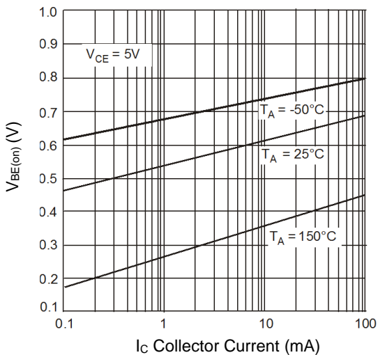
Figure 6. V_{BE(on)} \text{ v } I_C
