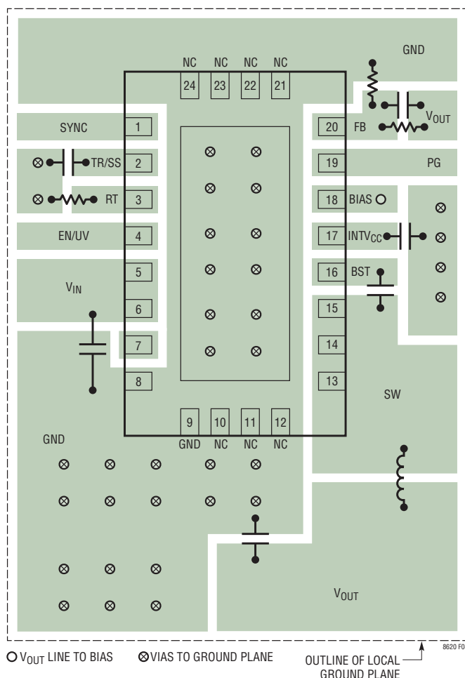
Figure 4b. Recommended PCB Layout for the LT8620 QFN Package
