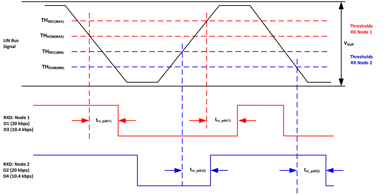
Figure 7-14. Propagation Delay
