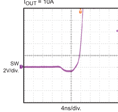
Dead Time (on) I_{OUT} = 10A
