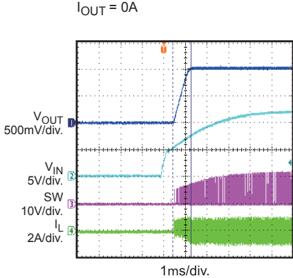
Start Up Through V_{IN} I_{OUT} = 0A
