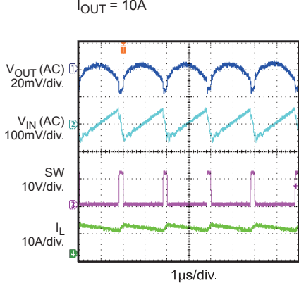
Input/Output Voltage Ripple I_{OUT} = 10A
