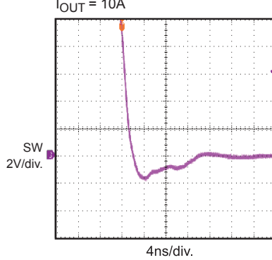
Dead Time (off) I_{OUT} = 10A
