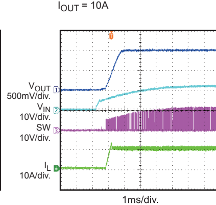
Start Up Through V_{IN} I_{OUT} = 10A
