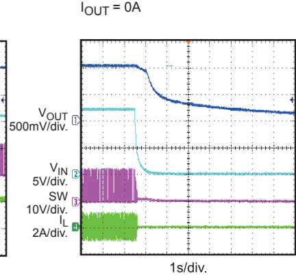
Shutdown Through V_{IN} I_{OUT} = 0A
