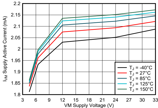
Figure 7-3. Active Current ( I_{VM} ) vs. Supply Voltage ( V_{VM} )
