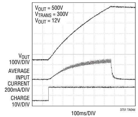
Charging Waveform
