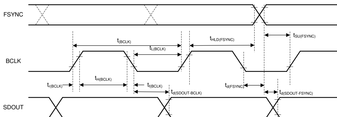
Figure 7-3. TDM, I²S, LJ Interface Timing Diagram
