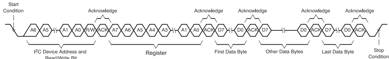
Figure 8-72. I 2 C Multiple-Byte Write Transfer
