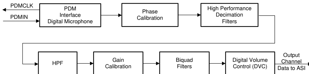
Figure 8-22. Digital PDM Input Signal-Chain Processing Flowchart
