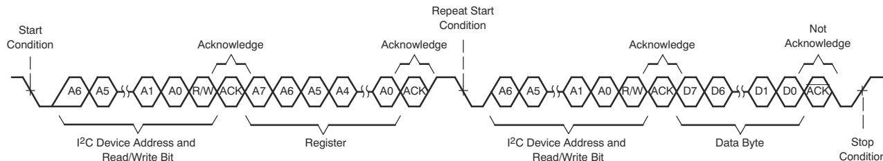
Figure 8-73. I 2 C Single-Byte Read Transfer
