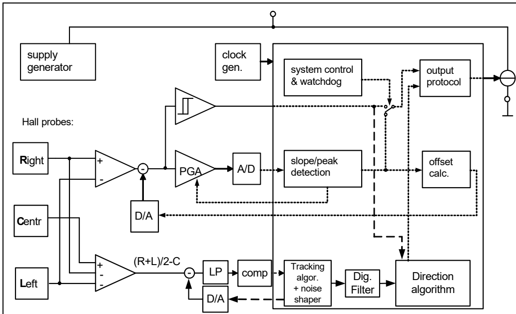
Figure 2-1 Block Diagram
