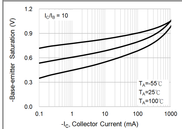
Fig.8 Base-Emitter Saturation Voltage (-25)
