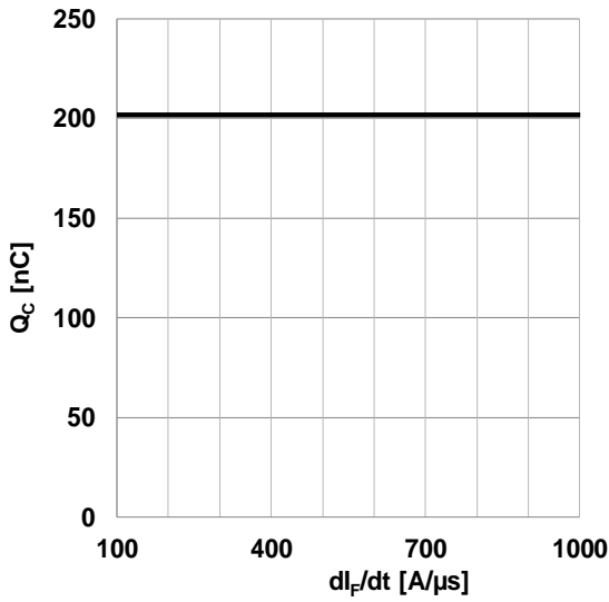
Figure 5. Typical capacitive charge as function of current slope 2 , Q_C=f(dI_F/dt) , T_{vj}=150^{\circ}C
