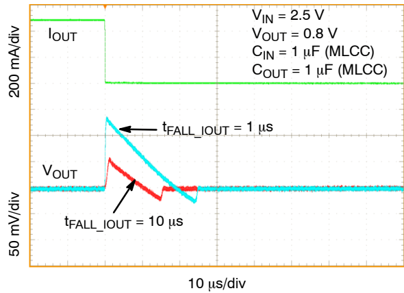
Figure 55. Load Transient Response – Falling Edge, V_{OUT} = 0.8\text{ V} , I_{OUT} = 1\text{ mA} to 500\text{ mA} , t_{FALL\_IOUT} = 1\text{ }\mu\text{s} , 10\text{ }\mu\text{s}
