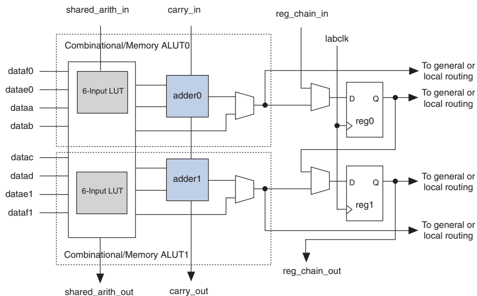
Figure 2-5. High-Level Block Diagram of the Stratix IV ALM
