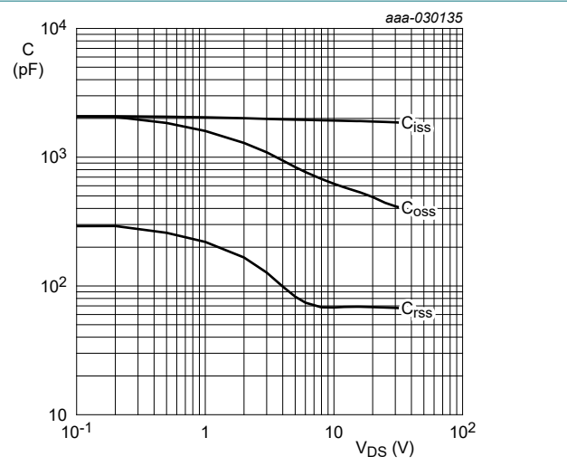
V_{GS} = 0 \text{ V}; f = 1 \text{ MHz} Fig. 15. Input, output and reverse transfer capacitances as a function of drain-source voltage; typical values
