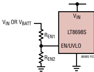
Figure 7. UVLO Divider
