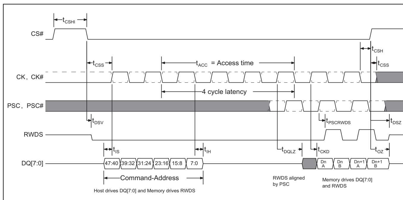
Figure 9 HYPERFLASH™ Read DCARS timing diagram [17, 18, 19, 20]
