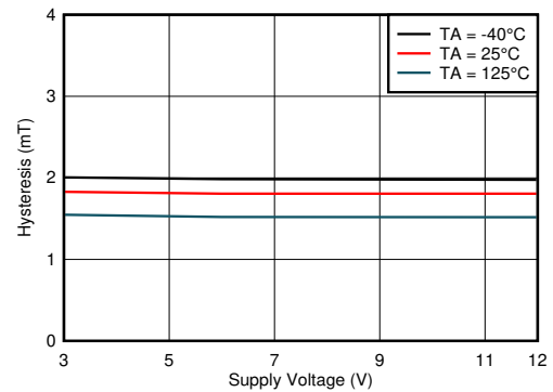
Figure 7-12. Hysteresis vs V CC
