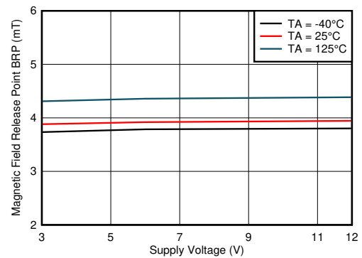
Figure 7-10. B RP vs V CC
