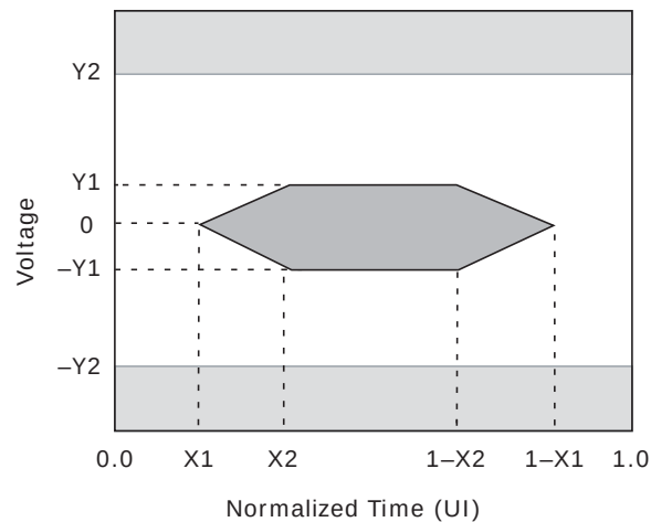
Figure 90 • SFI Transmit Differential Output Compliance Mask
