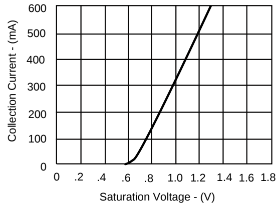
Figure 8 • Output Characteristics
