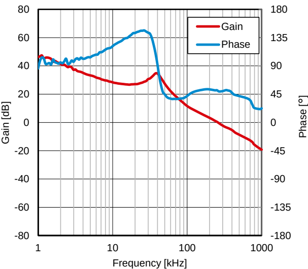
Figure 66. Frequency Characteristics ( I_{OUT} = 3.0\text{ A} )
