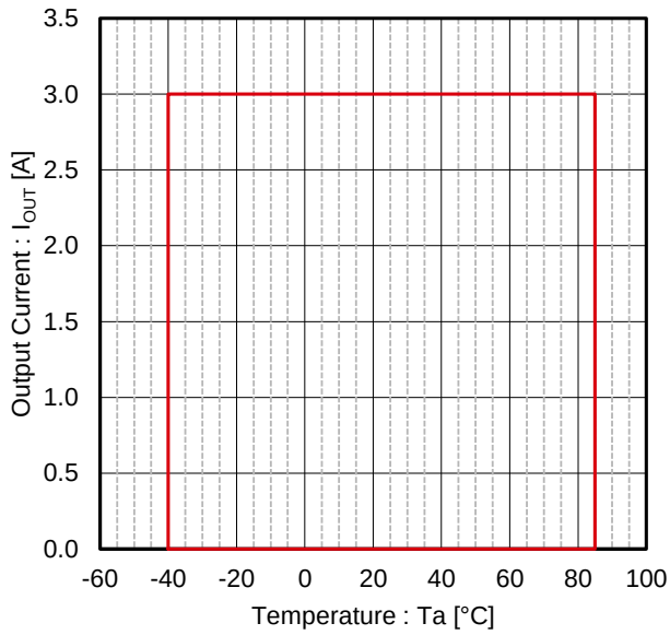
Figure 25. Output Current vs Temperature (Note 1) Operating Range: T_j < 150^\circ\text{C} ( V_{IN} = 5.0\text{ V} , V_{OUT} = 1.8\text{ V} )
