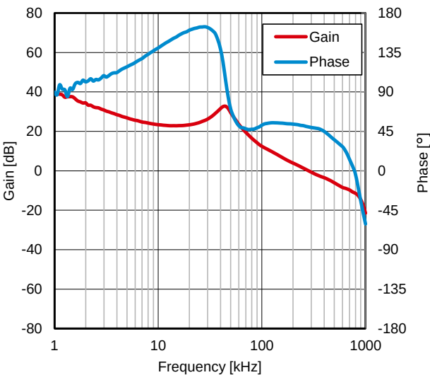
Figure 51. Frequency Characteristics ( I_{OUT} = 3.0\text{ A} )
