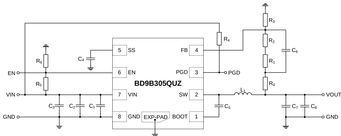
Figure 53. Application Circuit
