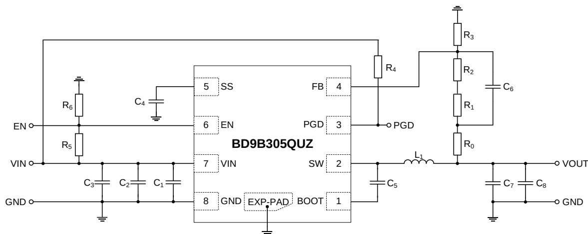
Figure 58. Application Circuit
