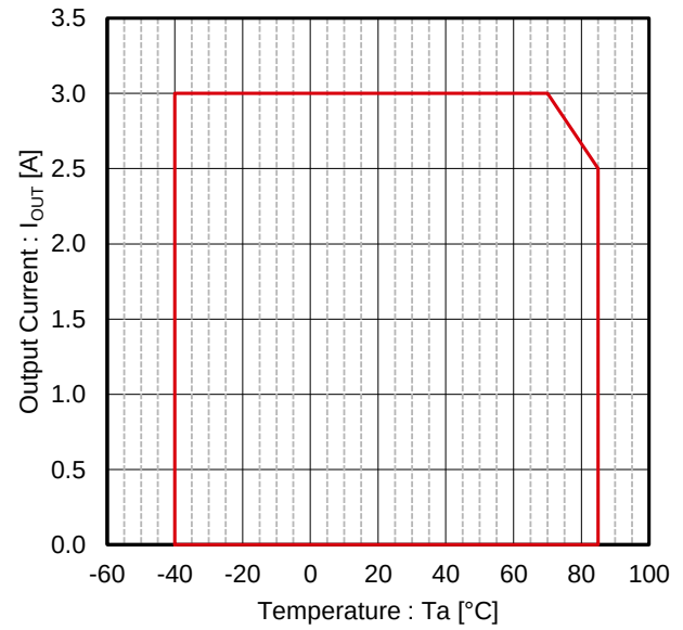
Figure 26. Output Current vs Temperature (Note 1) Operating Range: T_j < 150^\circ\text{C} ( V_{IN} = 3.3\text{ V} , V_{OUT} = 1.8\text{ V} )
