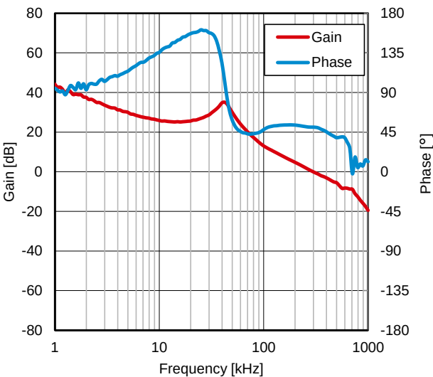
Figure 56. Frequency Characteristics ( I_{OUT} = 3.0\text{ A} )
