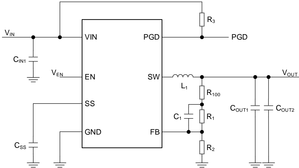
Figure 29. Reference Circuit 1
