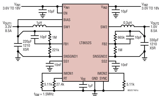
3.3V/8.5A, 1.0V/8.5A 1.5MHz Step-Down Converter
