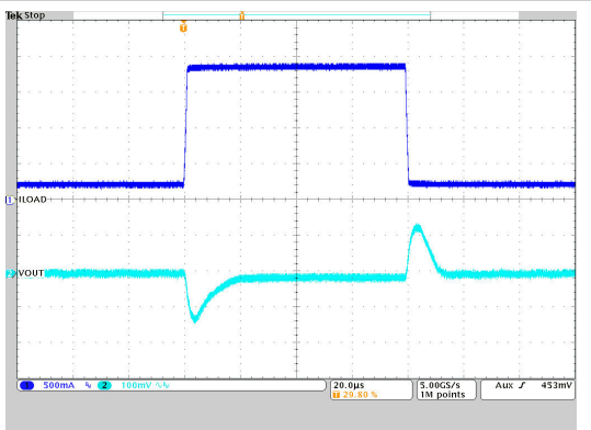
Figure 9-22. Load Transient Response
