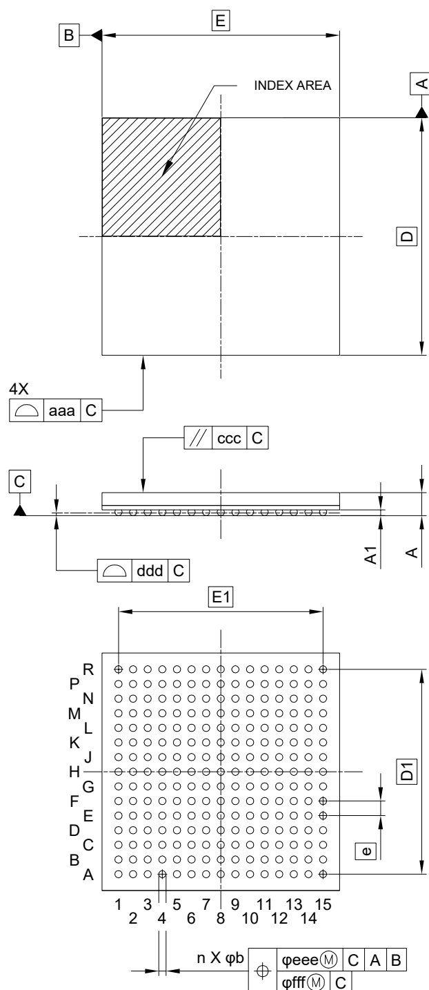
Figure 1.1 225 pin FBGA
