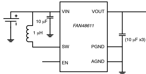
Figure 1. Typical Application
