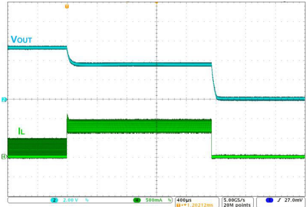
Figure 14. Overload Protection
