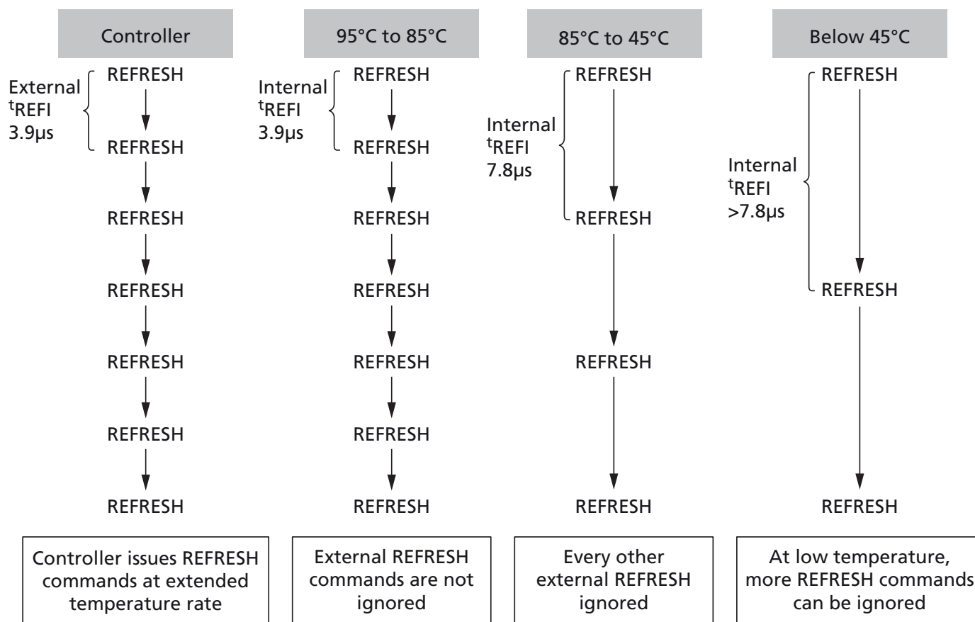
Figure 78: TCR Mode Example 1
