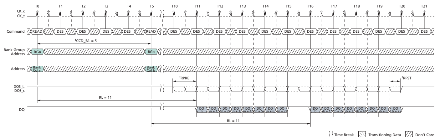
Figure 126: Nonconsecutive READ (BL8) with 1 st CK Preamble in Same or Different Bank Group
