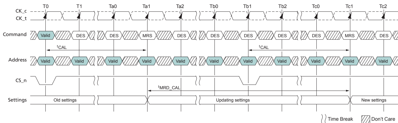
Figure 24: t_{MRD\_CAL} , Mode Register Cycle Time With CAL Enabled
