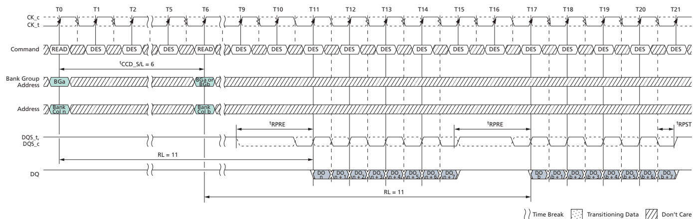
Figure 127: Nonconsecutive READ (BL8) with 2 nd CK Preamble in Same or Different Bank Group
