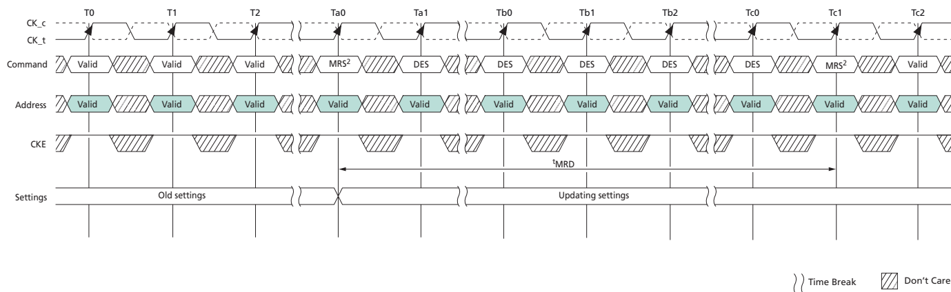
Figure 10: t^{\text{MRD}} Timing
