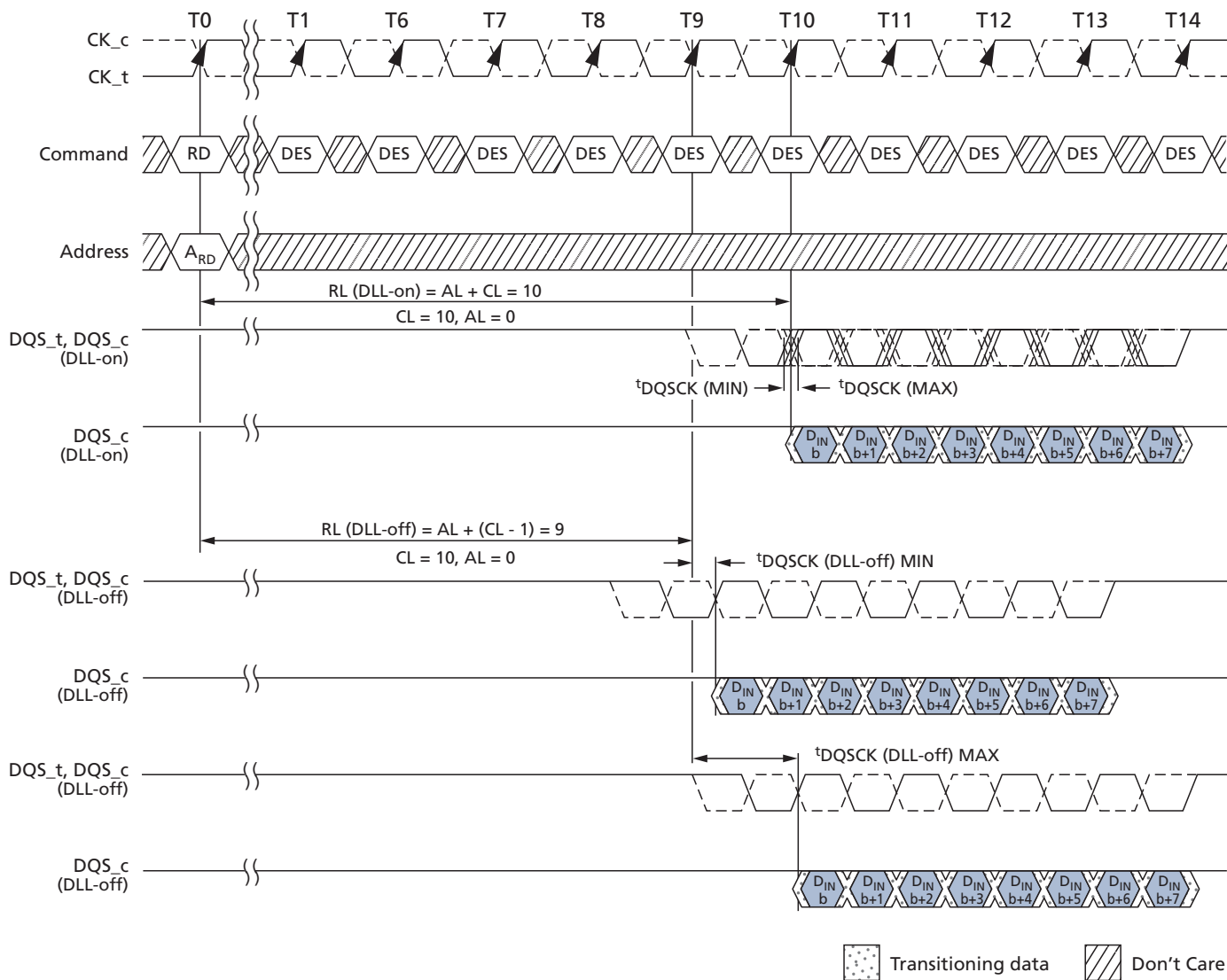
Figure 12: DLL-Off Mode Read Timing Operation
