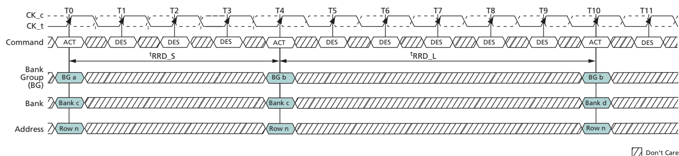
Figure 73: t_{RRD} Timing
