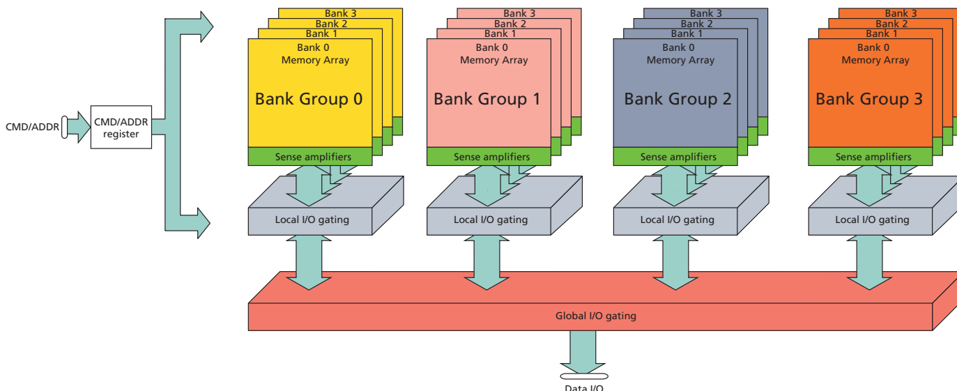
Figure 110: Bank Group x4/x8 Block Diagram
