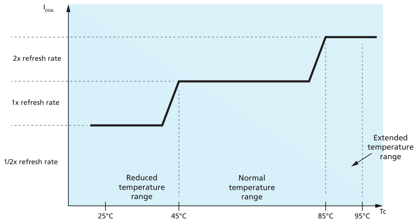
Figure 27: Auto Self Refresh Ranges
