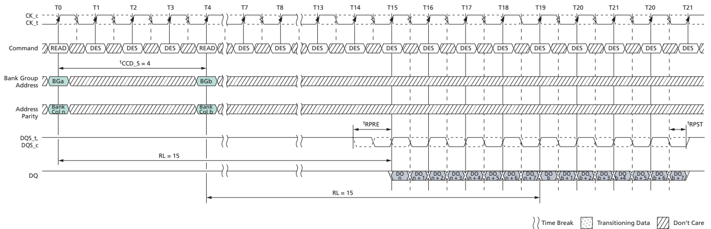
Figure 150: Consecutive READ (BL8) with 1 st CK Preamble and CA Parity in Different Bank Group
