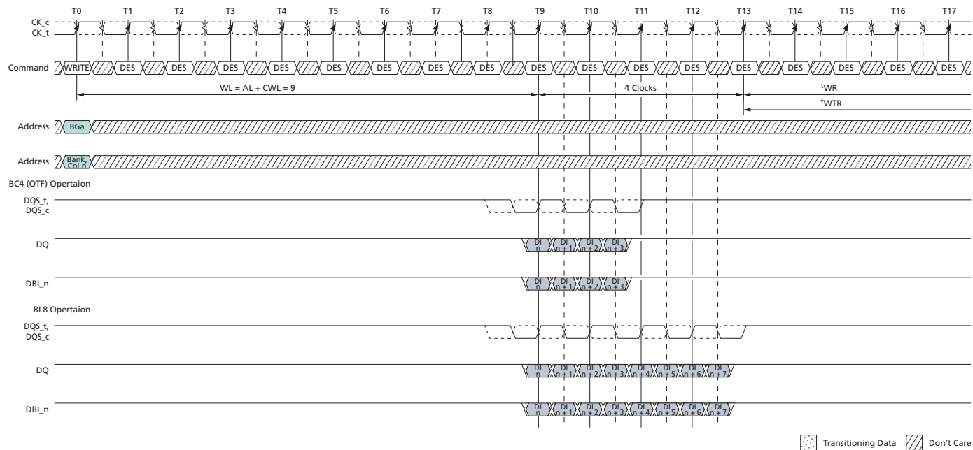
Figure 183: WRITE (BL8/BC4-OTF) with 1 t CK Preamble and DBI
