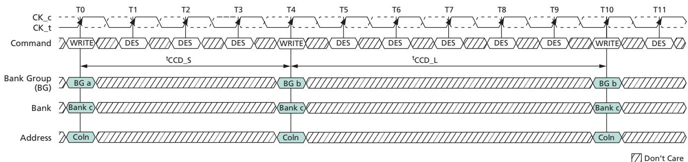
Figure 112: Write Burst t_{CCD\_S} and t_{CCD\_L} Examples
