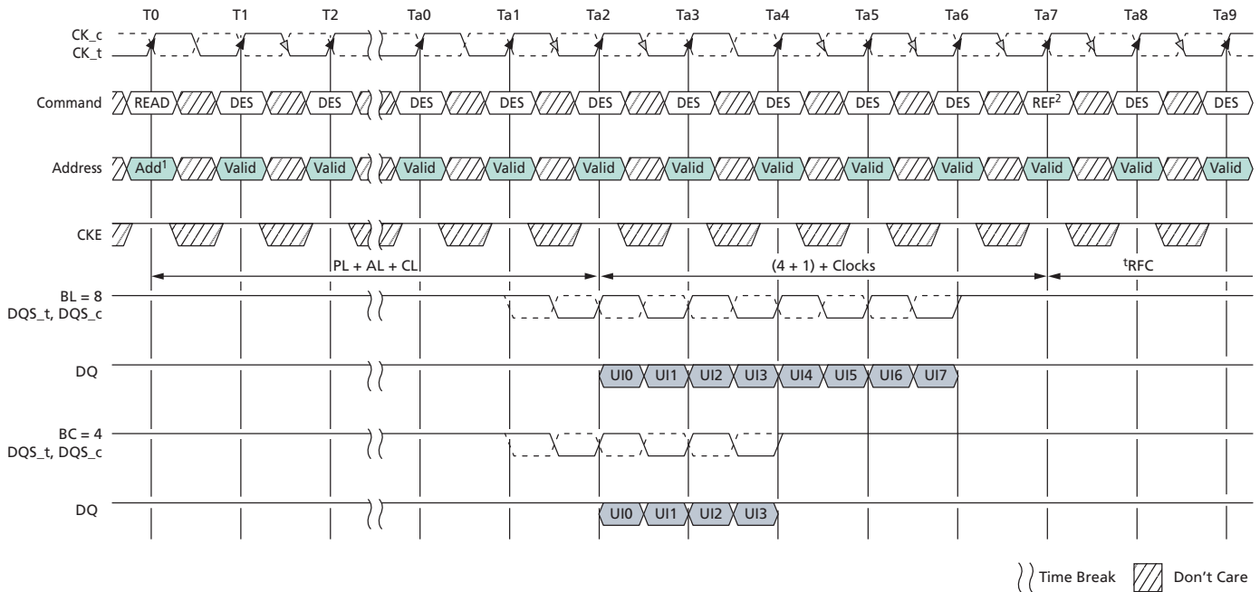
Figure 35: READ-to-REFRESH Timing
