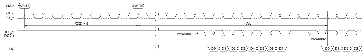
Figure 105: 1 t CK vs. 2 t CK WRITE Preamble Mode, t_{CCD} = 6
