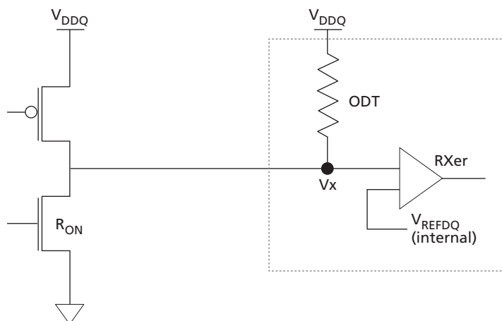
Figure 66: V_{\text{REFDQ}} Equivalent Circuit
