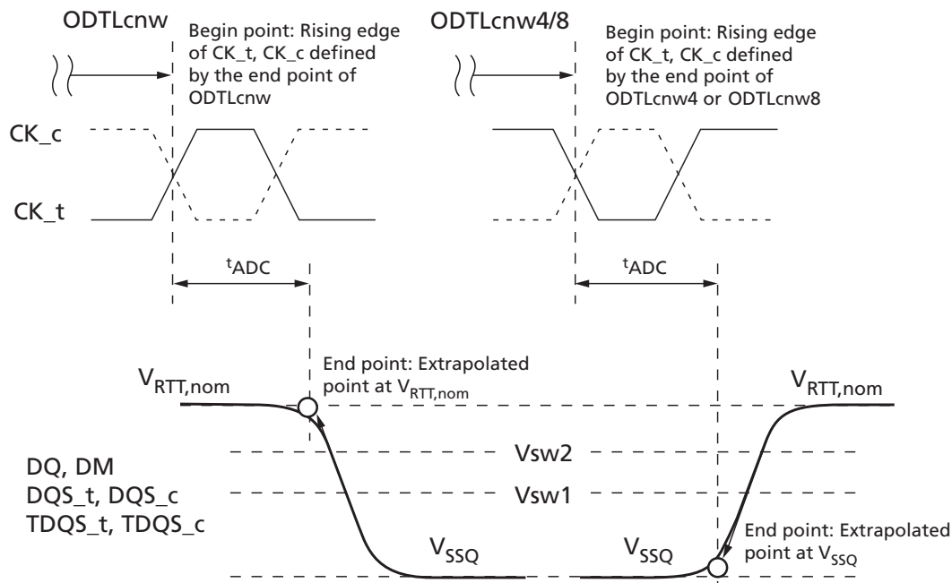
Figure 231: t_{ADC} Definition with Dynamic ODT Control
