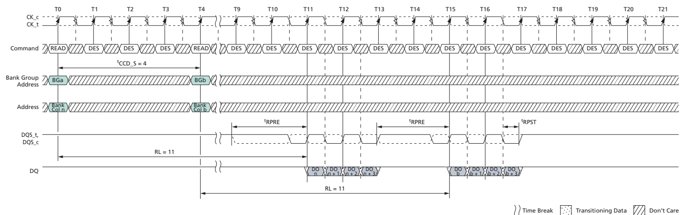
Figure 129: READ (BC4) to READ (BC4) with 2 nd CK Preamble in Different Bank Group
