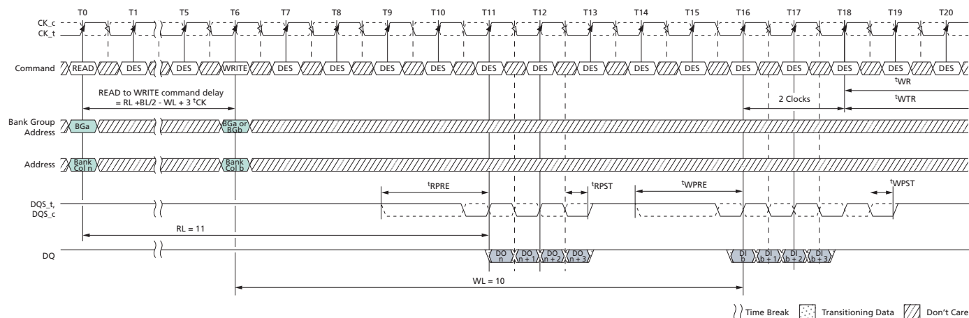
Figure 139: READ (BC4) Fixed to WRITE (BC4) Fixed with 2^t\text{CK} Preamble in Same or Different Bank Group
