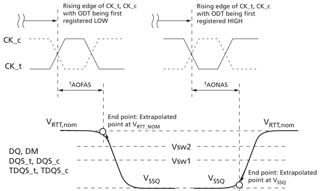
Figure 232: t_{\text{AOFAS}} and t_{\text{AONAS}} Definitions
