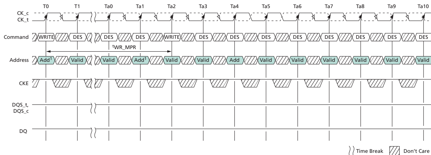
Figure 33: MPR Back-to-Back WRITE Timing
