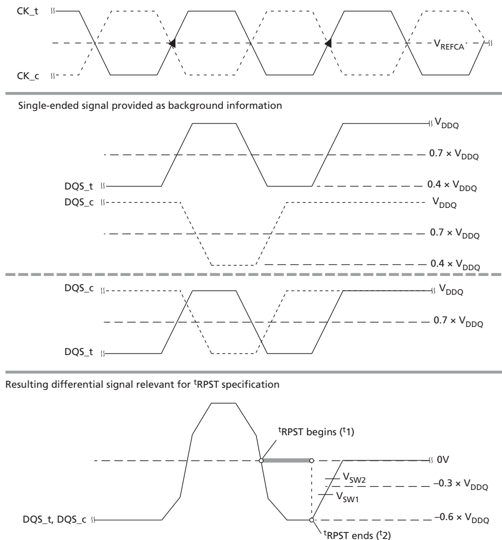
Figure 121: t_{RPST} Method for Calculating Transitions and Endpoints
