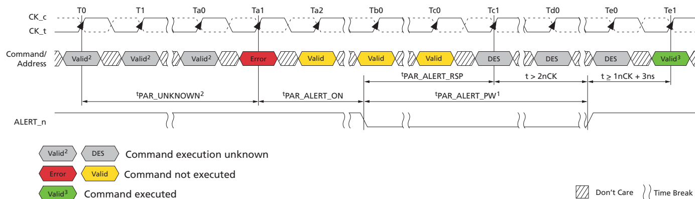
Figure 46: Persistent CA Parity Error Checking Operation
