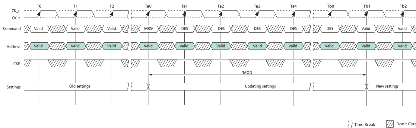
Figure 11: t^{\text{MOD}} Timing
