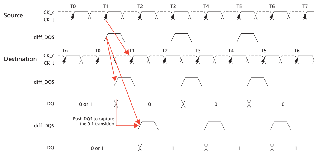
Figure 15: Write-Leveling Concept, Example 1
