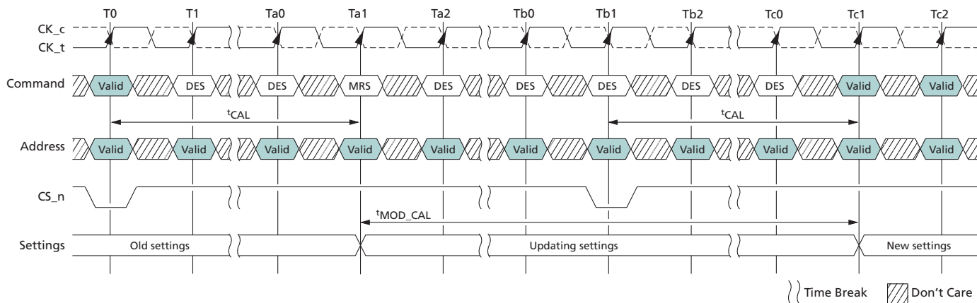
Figure 22: t_{MOD\_CAL} , MRS to Valid Command Timing with CAL Enabled
