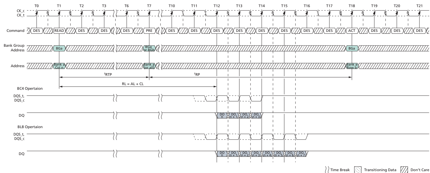
Figure 144: READ to PRECHARGE with 1 t CK Preamble
