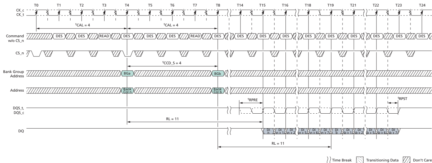
Figure 155: Consecutive READ (BL8) with CAL ( 4^t\text{CK} ) and 1^t\text{CK} Preamble in Different Bank Group
