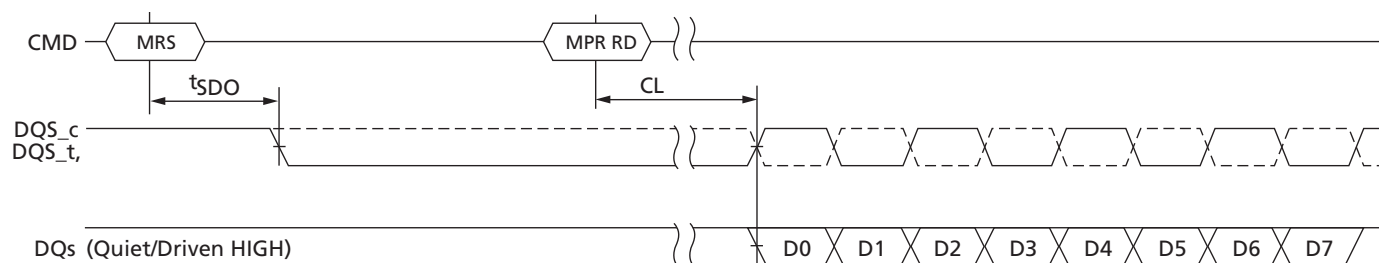
Figure 107: READ Preamble Training
