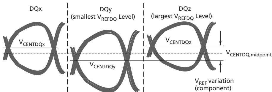
Figure 158: V_{\text{CENT\_DQ}} V_{\text{REFDQ}} Voltage Variation
