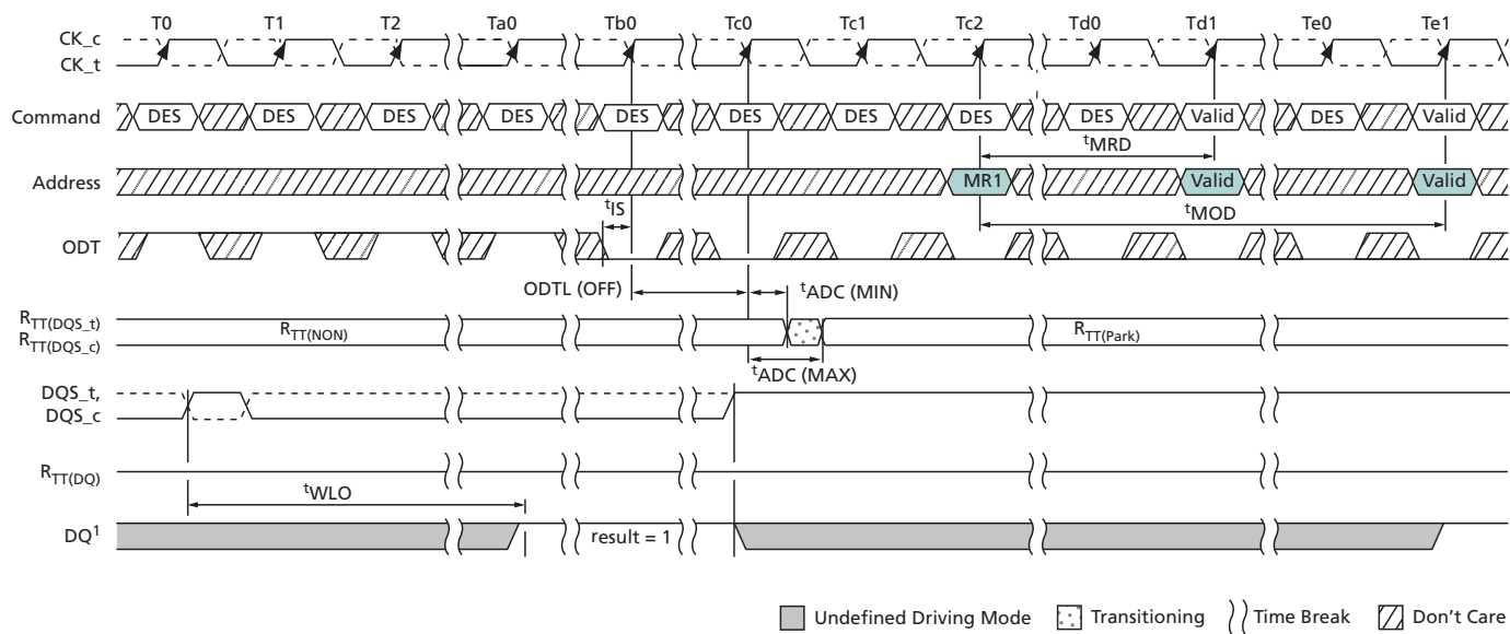
Figure 18: Write-Leveling Exit
