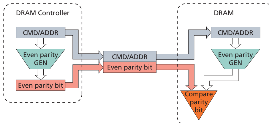
Figure 44: Command/Address Parity Operation
