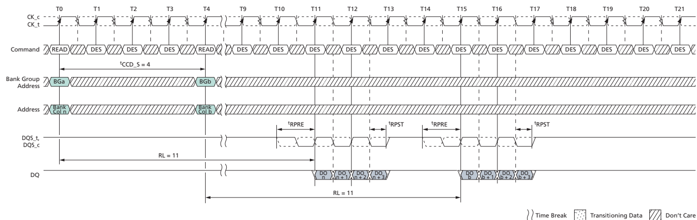
Figure 128: READ (BC4) to READ (BC4) with 1 st CK Preamble in Different Bank Group
