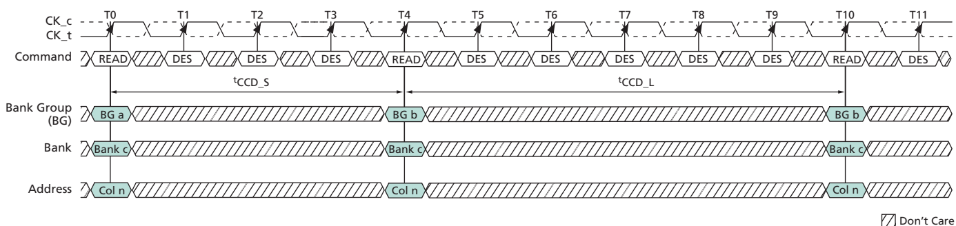
Figure 111: READ Burst t_{CCD\_S} and t_{CCD\_L} Examples
