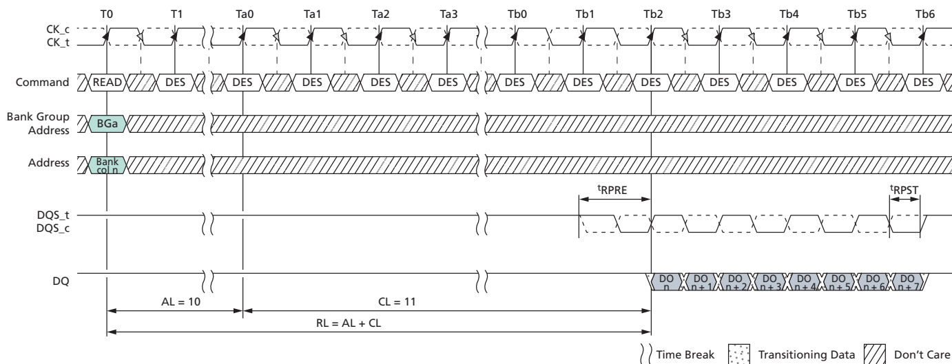
Figure 123: READ Burst Operation, RL = 21 (AL = 10, CL = 11, BL8)
