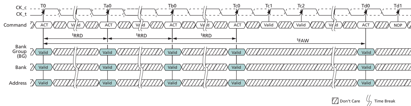
Figure 74: t_{FAW} Timing
