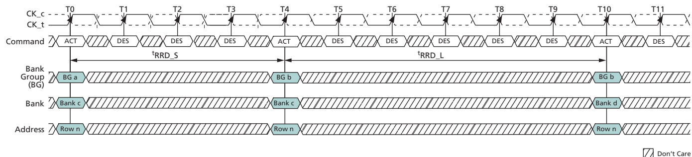
Figure 113: t_{RRD} Timing
