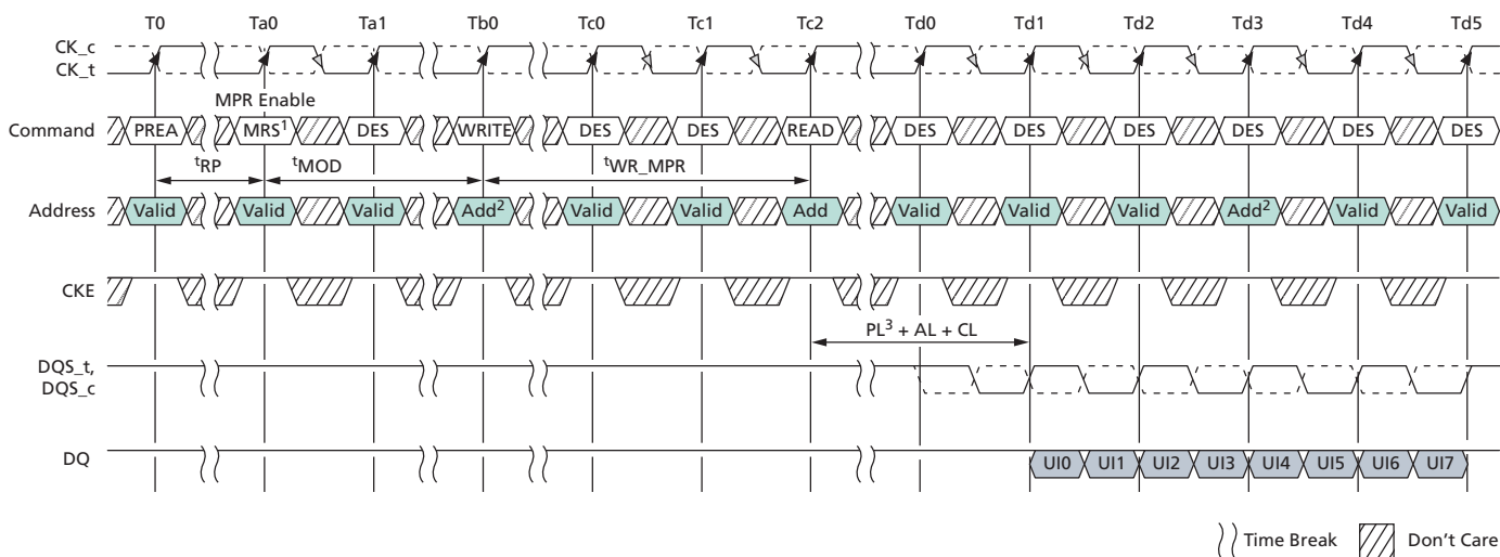
Figure 32: MPR WRITE and WRITE-to-READ Timing
