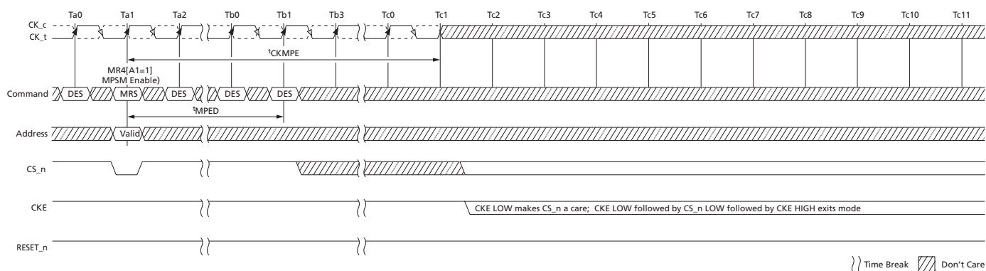
Figure 40: Maximum Power-Saving Mode Entry
