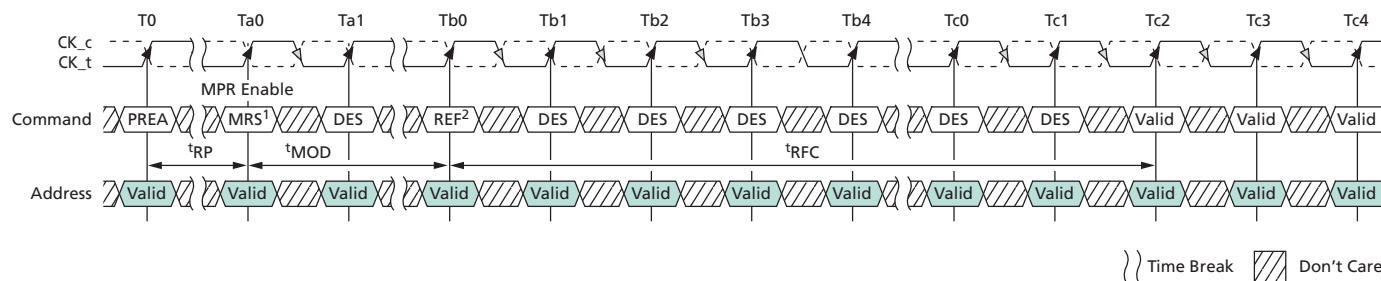
Figure 34: REFRESH Timing
