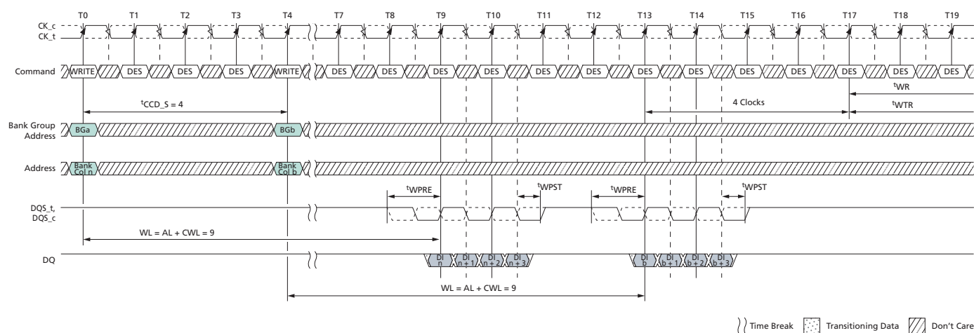
Figure 168: WRITE (BC4) OTF to WRITE (BC4) OTF with 1^tCK Preamble in Different Bank Group
