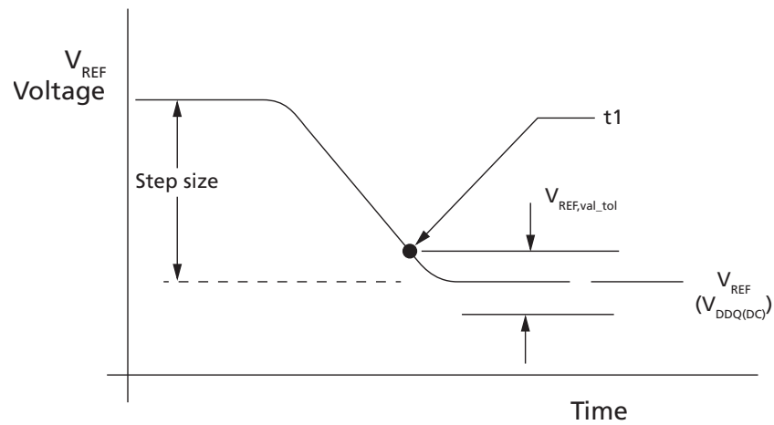
Figure 63: V REF Step: Single Step Size Decrement Case
