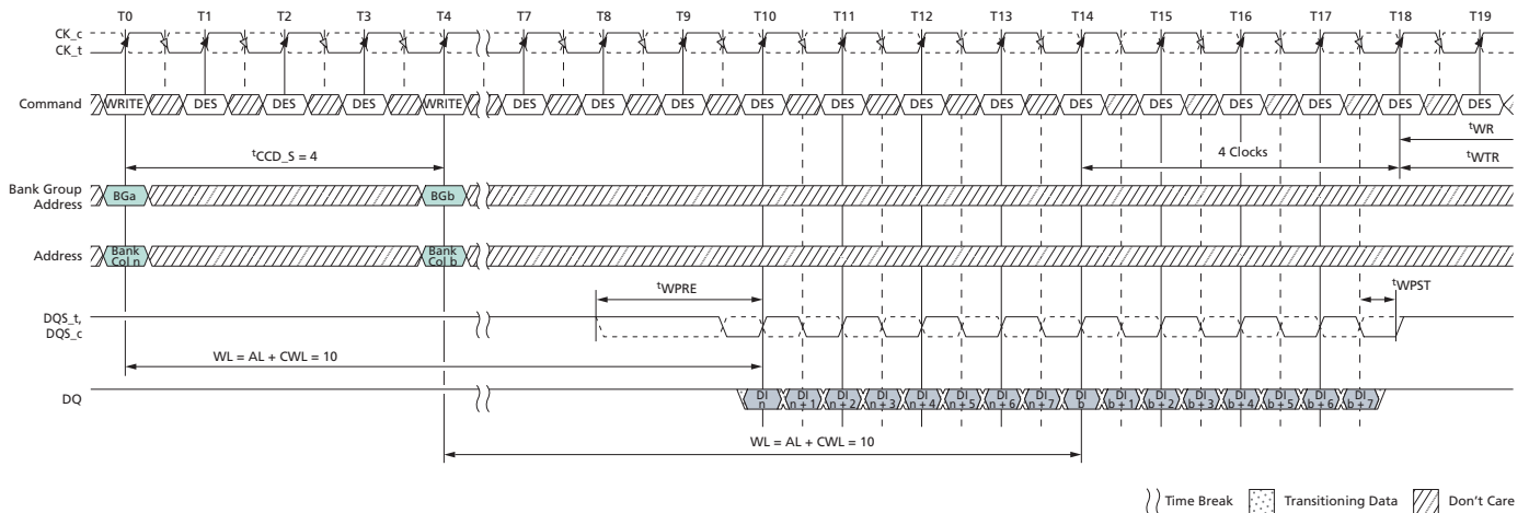
Figure 165: Consecutive WRITE (BL8) with 2^t\text{CK} Preamble in Different Bank Group
