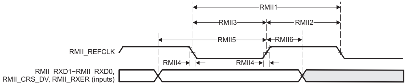
Figure 5-30. EMAC Receive Interface Timing RMII operation
