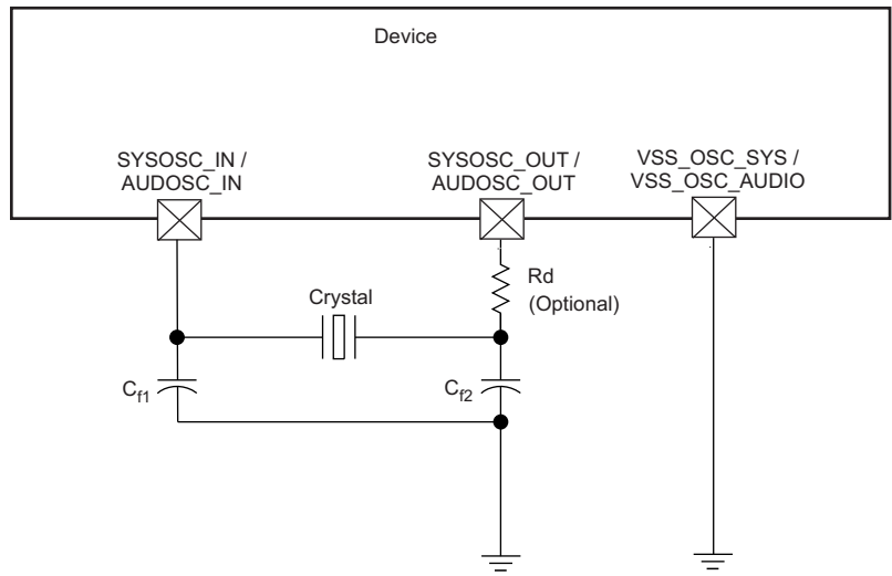
Figure 7-26. Grounding Scheme for internal oscillators
