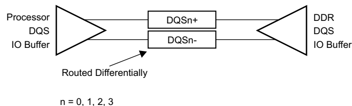
Figure 7-16. DQS Topology
