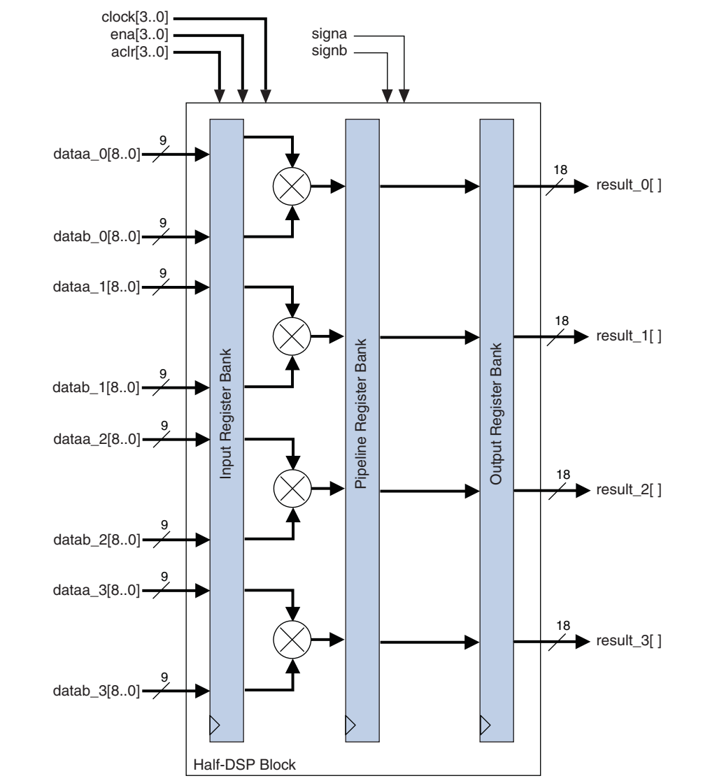
Figure 4-10. 9-Bit Independent Multiplier Mode Shown for a Half Block
