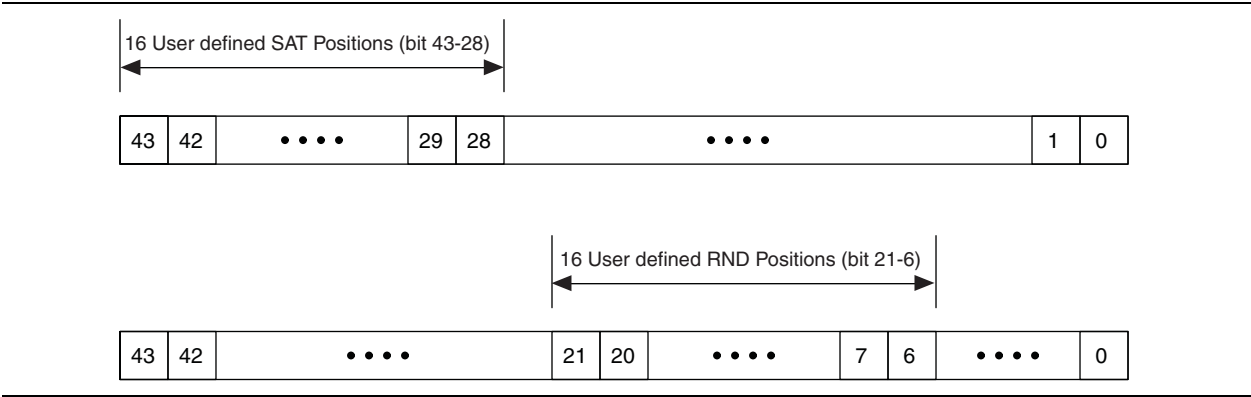
Figure 4-21. Rounding and Saturation Locations
