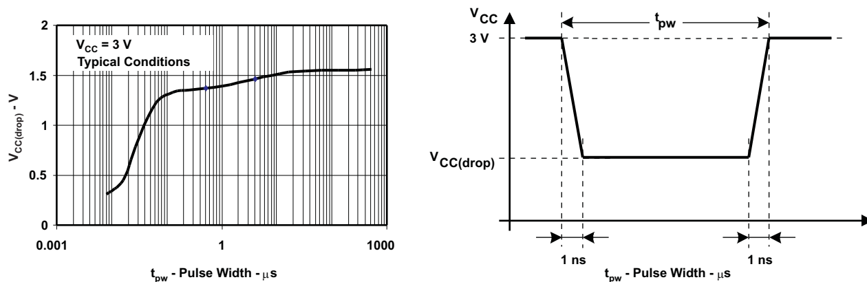
Figure 5-8. V_{CC(drop)} Level with a Square Voltage Drop to Generate a POR or BOR Signal
