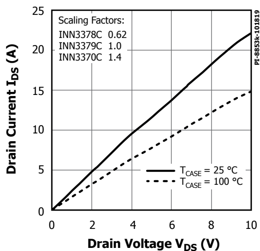
Figure 53. Output Characteristics.
