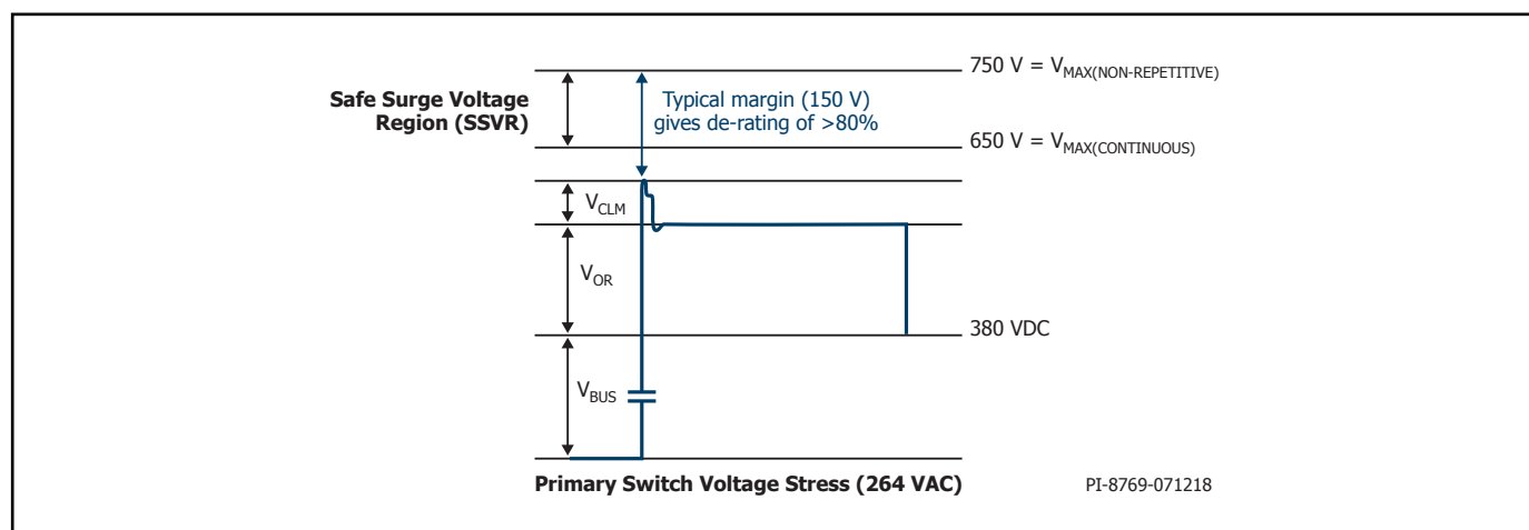
Figure 39. Peak Drain Voltage for 264 VAC Input Voltage.
