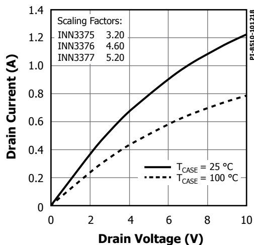
Figure 49. Output Characteristics.
