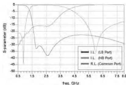
RFDIP2520100G2T
