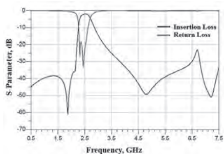
RFBPF2012080A7T
