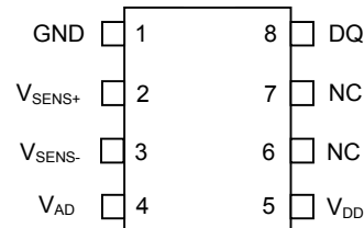
DS2438Z, DS2438AZ 8-Pin SOIC (150-mil)
