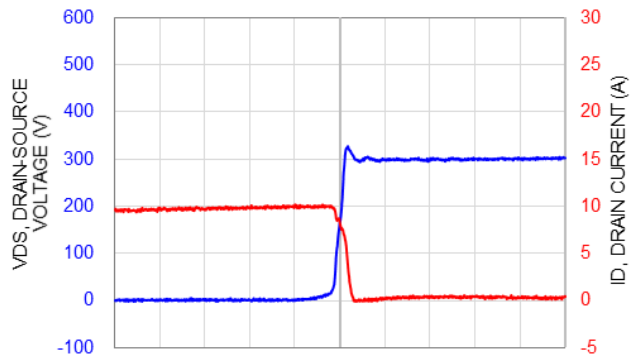
Figure 11. Turn-off Waveform T_J = 100\text{ }^\circ\text{C} , V_{PN} = 300\text{ V}
