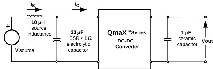
Fig. 1.8V.11: Test Setup for measuring input reflected ripple currents, i_c and i_s .
