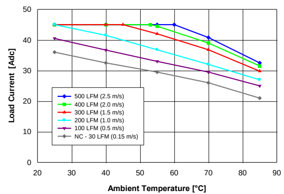
Fig. 3.3V.2: Available load current vs. ambient air temperature and airflow rates for QM48T45033 converter with B height pins mounted horizontally with V_{in} = 48\text{ V} , air flowing from pin 3 to pin 1, and MOSFET temperature \leq 120^\circ\text{C} .
