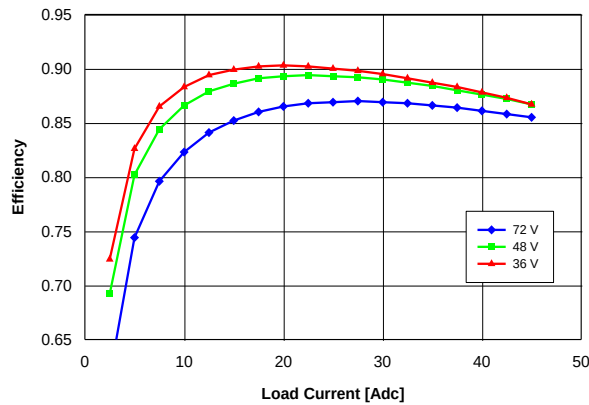
Fig. 1.8V.3: Efficiency vs. load current and input voltage for converter mounted vertically with air flowing from pin 3 to pin 1 at a rate of 300 LFM (1.5 m/s) and T_a = 25^\circ\text{C} .
