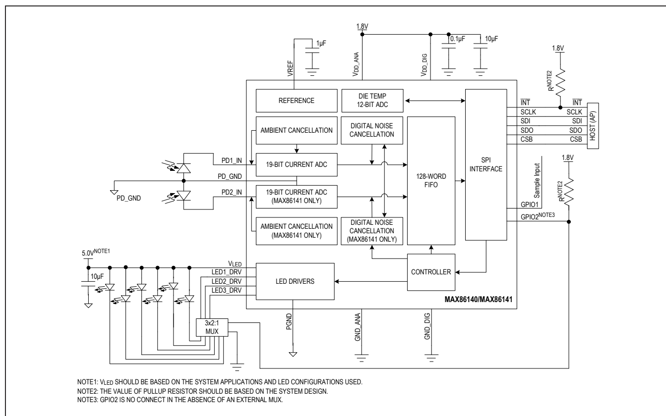
Figure 10. Block Diagram for GPIO CTRL[3:0] 0010 with External Mux
