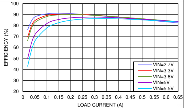
Figure 8-3. Efficiency V_{OUT} = 1.2\text{ V}
