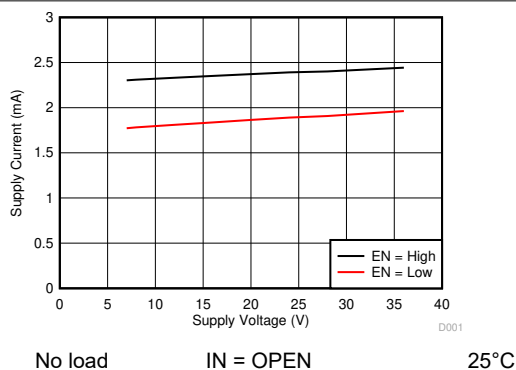
Figure 6-1. Supply Current vs Supply Voltage
