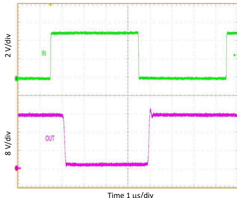
Figure 9-4. OUT in Push-Pull Mode
