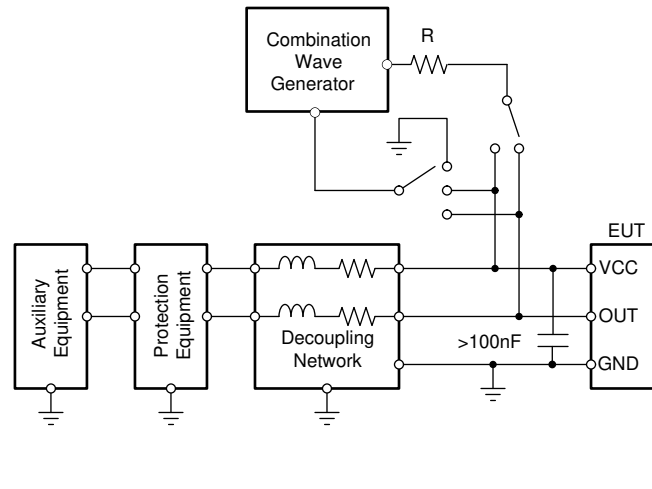
Figure 8-6. Surge Test Setup
