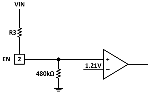
Figure 24. Programming UVLO
