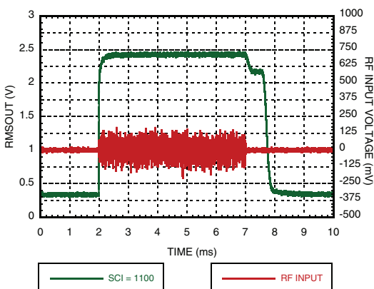
Figure 7. Residual Ripple for 1900 MHz WCDMA4C @ SCI=1100
