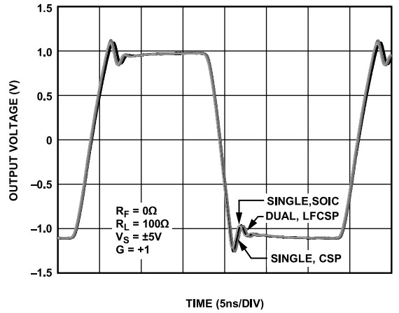
Figure 23. Large Signal Transient Response vs. Package
