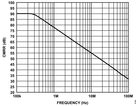
Figure 26. Common-Mode Rejection Ratio (CMRR) vs. Frequency
