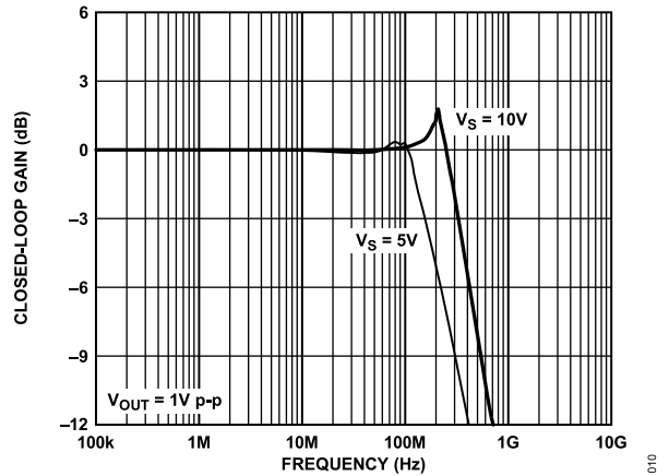
Figure 12. Large Signal Frequency Response for Various Supplies
