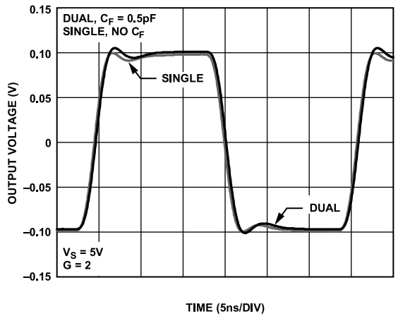
Figure 22. Small Signal Transient Response
