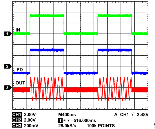
Figure 58. Power-Down Operation
