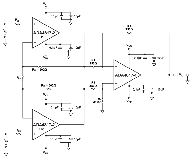
Figure 66. High Speed Instrumentation Amplifier
