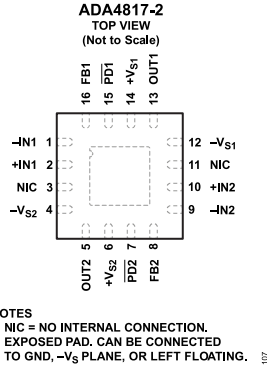
Figure 7. ADA4817-2 Pin Configuration (16-Lead LFCSP)
