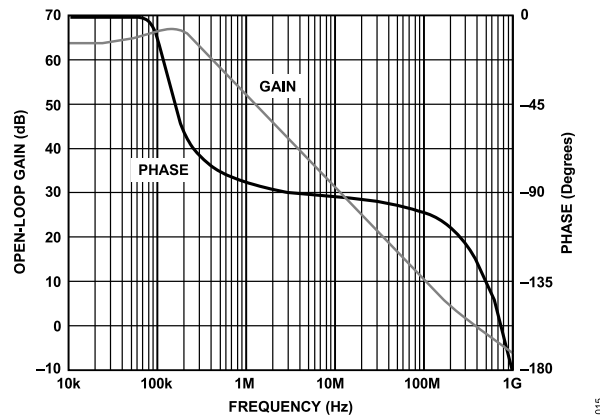
Figure 31. Open-Loop Gain and Phase vs. Frequency
