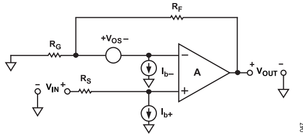
Figure 55. DC Errors of the Voltage Feedback Amplifier
