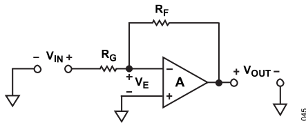
Figure 53. Inverting Configuration
