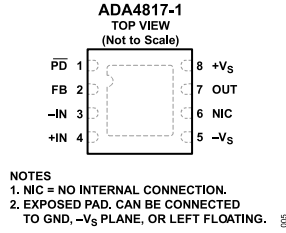
Figure 5. ADA4817-1 Pin Configuration (8-Lead LFCSP)
