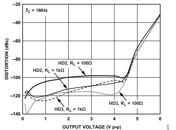
Figure 19. Distortion vs. Output Voltage for Various Loads
