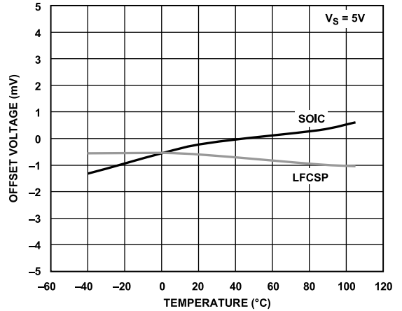
Figure 41. Offset Voltage vs. Temperature ( V_S = 5V )
