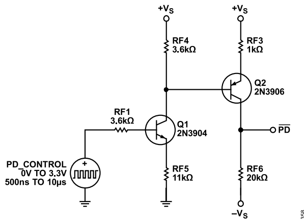
Figure 57. Power-Down Circuit
