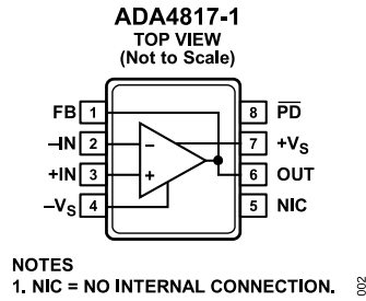
Figure 2. 8-Lead SOIC (RD-8-1)
