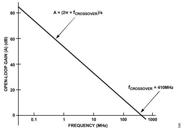
Figure 54. Open-Loop Gain vs. Frequency
