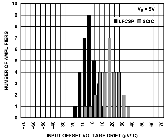
Figure 42. Input Offset Voltage Drift Histogram ( V_S = 5V )
