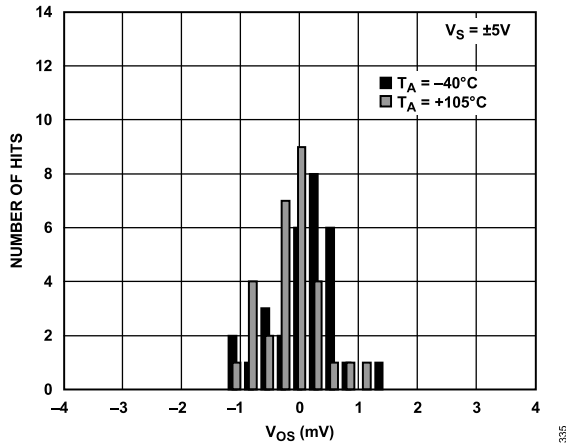
Figure 33. Input Offset Voltage Histogram over Temperature ( V_S = \pm 5 V ), LFCSP Only
