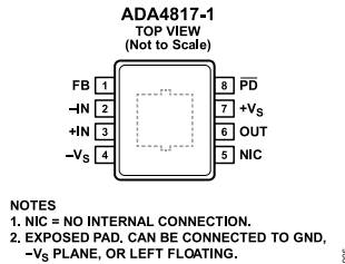
Figure 6. ADA4817-1 Pin Configuration (8-Lead SOIC)
