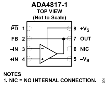
Figure 1. 8-Lead LFCSP (CP-8-13)
