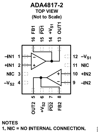
Figure 3. 16-Lead LFCSP (CP-16-20)
