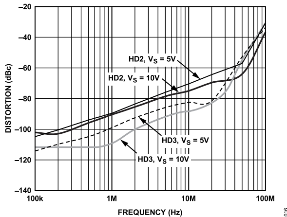
Figure 16. Distortion vs. Frequency for Various Supplies, G = 2 , V_{OUT} = 2\text{ V p-p}
