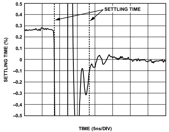
Figure 24. 0.1% Short-Term Settling Time
