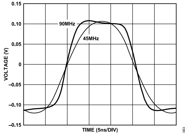
Figure 69. Small Signal Transient Response (Low-Pass Filter)
