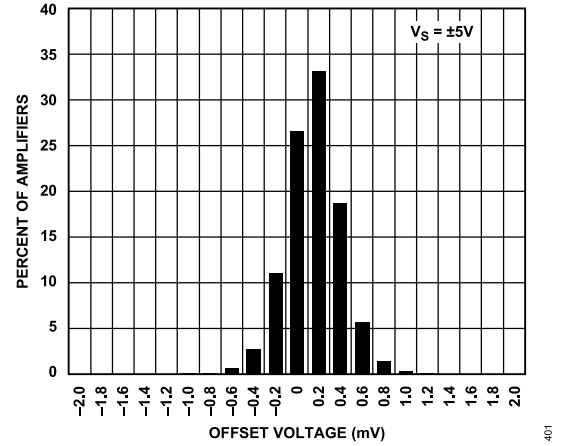
Figure 35. Input Offset Voltage Histogram ( V_S = \pm 5 V ), SOIC Only
