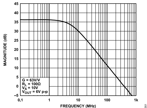
Figure 65. Photodiode Preamp Frequency Response
