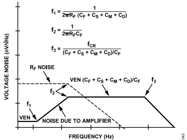
Figure 64. Photodiode Voltage Noise Contributions
