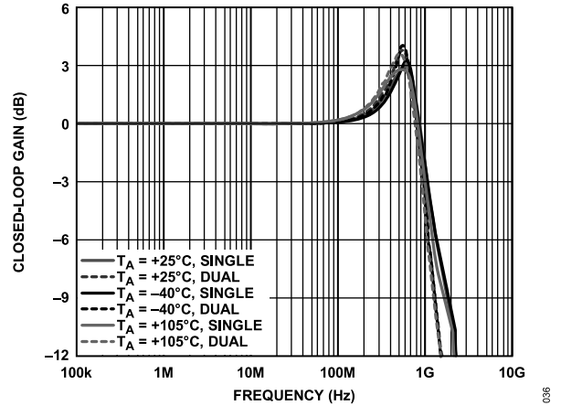
Figure 17. Small Signal Frequency Response vs. Temperature
