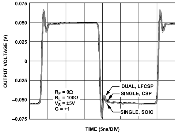
Figure 20. Small Signal Transient Response vs. Package
