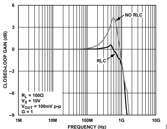
Figure 62. Frequency Response with RLC Circuit
