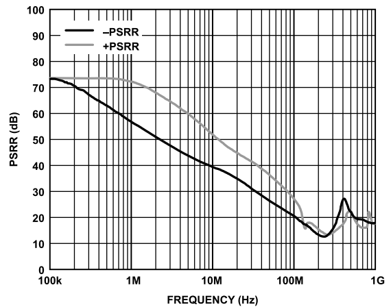
Figure 25. Power Supply Rejection Ratio (PSRR) vs. Frequency
