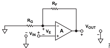
Figure 52. Noninverting Configuration
