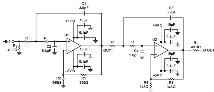
Figure 68. 4-Pole, Sallen-Key LPF (ADA4817-2)
