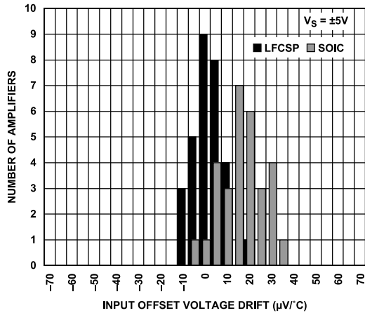
Figure 39. Input Offset Voltage Drift Histogram ( V_S = \pm 5V )
