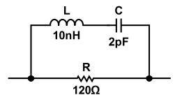
Figure 61. RLC Circuit
