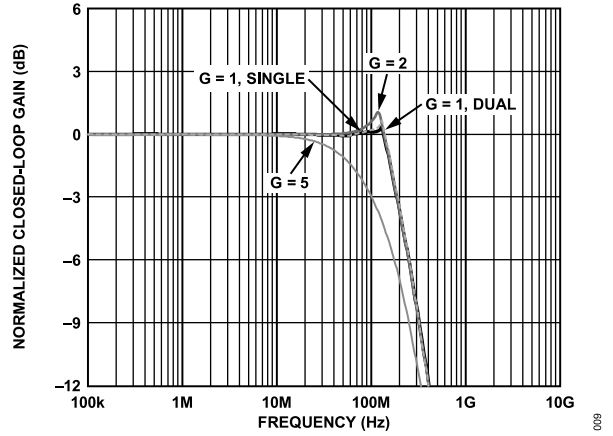
Figure 11. Large Signal Frequency Response for Various Gains
