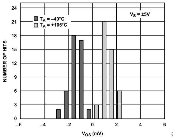
Figure 34. Input Offset Voltage Histogram over Temperature ( V_S = \pm 5 V ), SOIC Only
