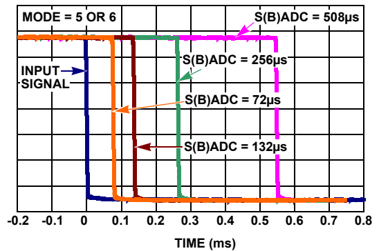
FIGURE 26. INTERRUPT TIMING
