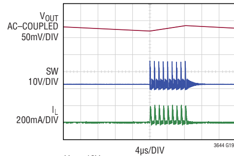
Pulse-Skipping Operation
