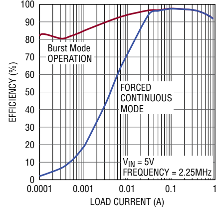
Efficiency vs Load at Dropout Operation
